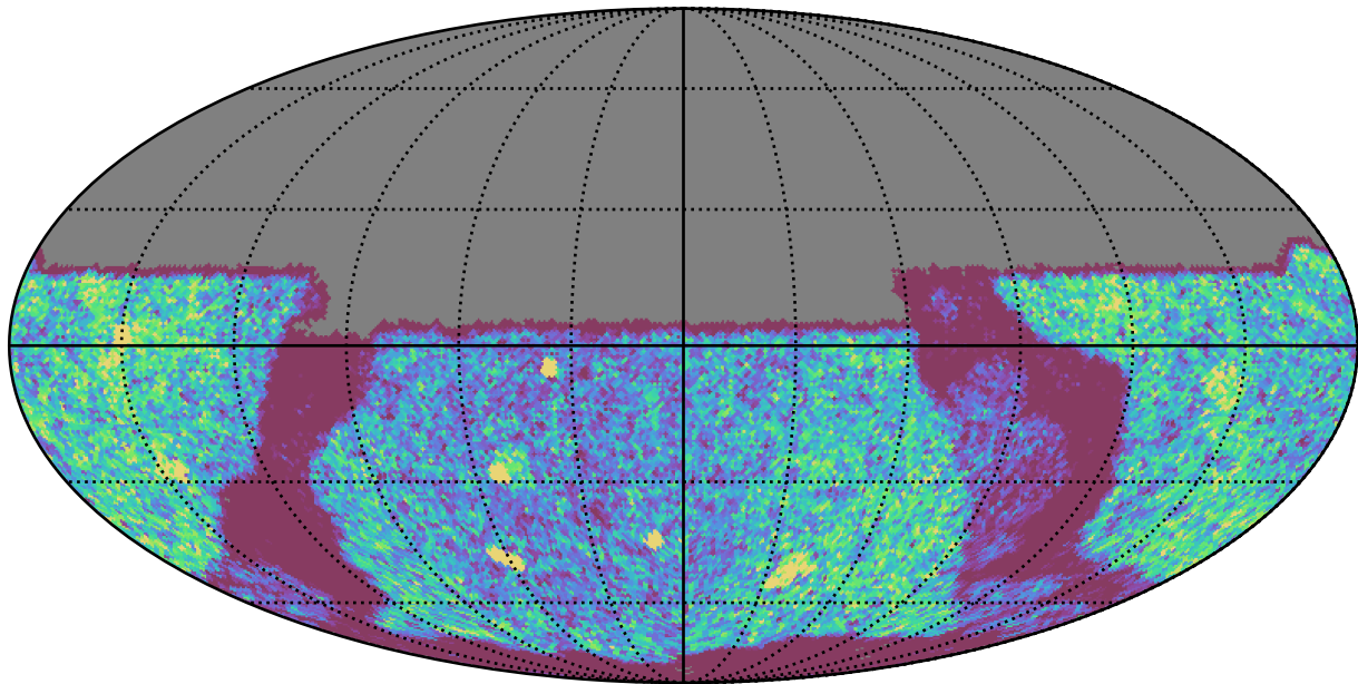
too_elab_heavy_r64_d3_ugrizy_v3.4_10yrs Yr 1 y band: NVisits
