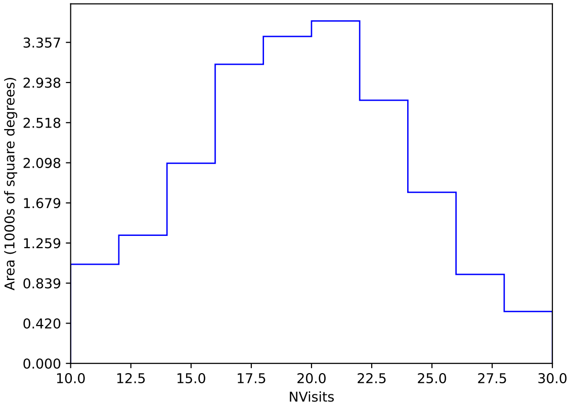
too_elab_heavy_r64_d3_ugrizy_v3.4_10yrs Yr 1 y band: NVisits
