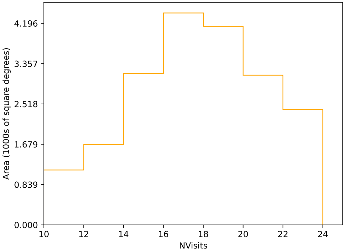
too_elab_heavy_r64_d3_ugrizy_v3.4_10yrs Yr 1 r band: NVisits
