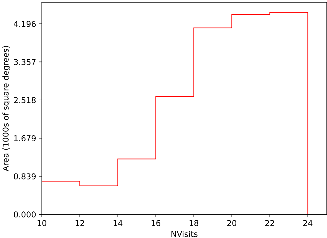
too_elab_heavy_r64_d3_ugrizy_v3.4_10yrs Yr 1 i band: NVisits
