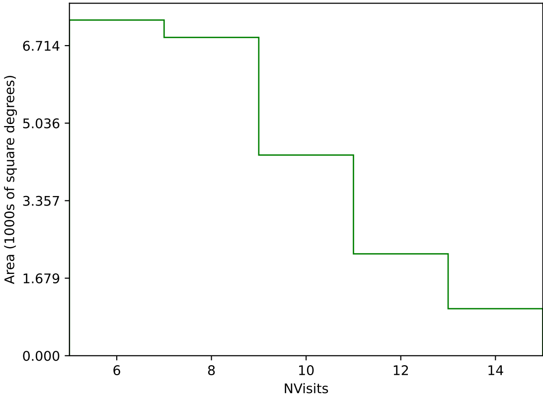
too_elab_heavy_r64_d3_ugrizy_v3.4_10yrs Yr 1 g band: NVisits
