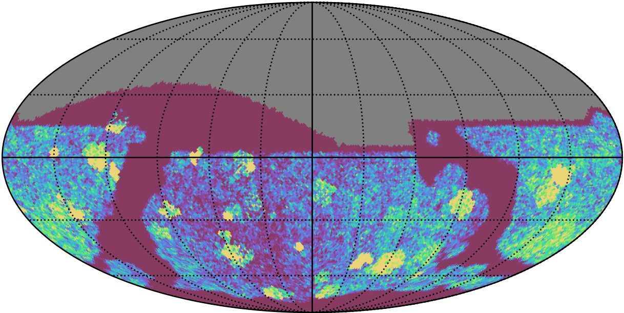
too_elab_heavy_r64_d3_ugrizy_v3.4_10yrs Yr 1 all bands: NVisits
