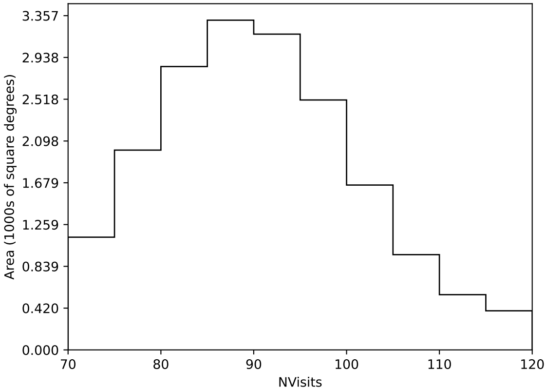
too_elab_heavy_r64_d3_ugrizy_v3.4_10yrs Yr 1 all bands: NVisits
