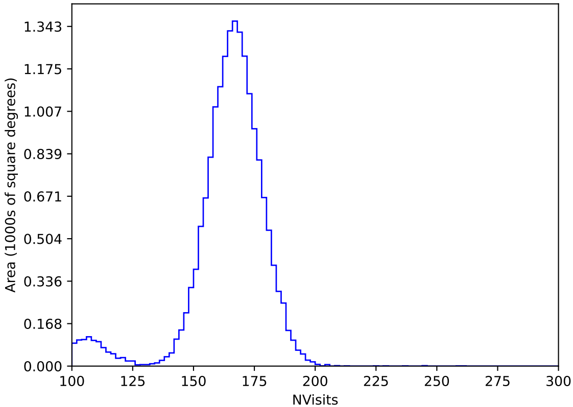
too_elab_heavy_r64_d3_ugrizy_v3.4_10yrs WFD y band: NVisits
