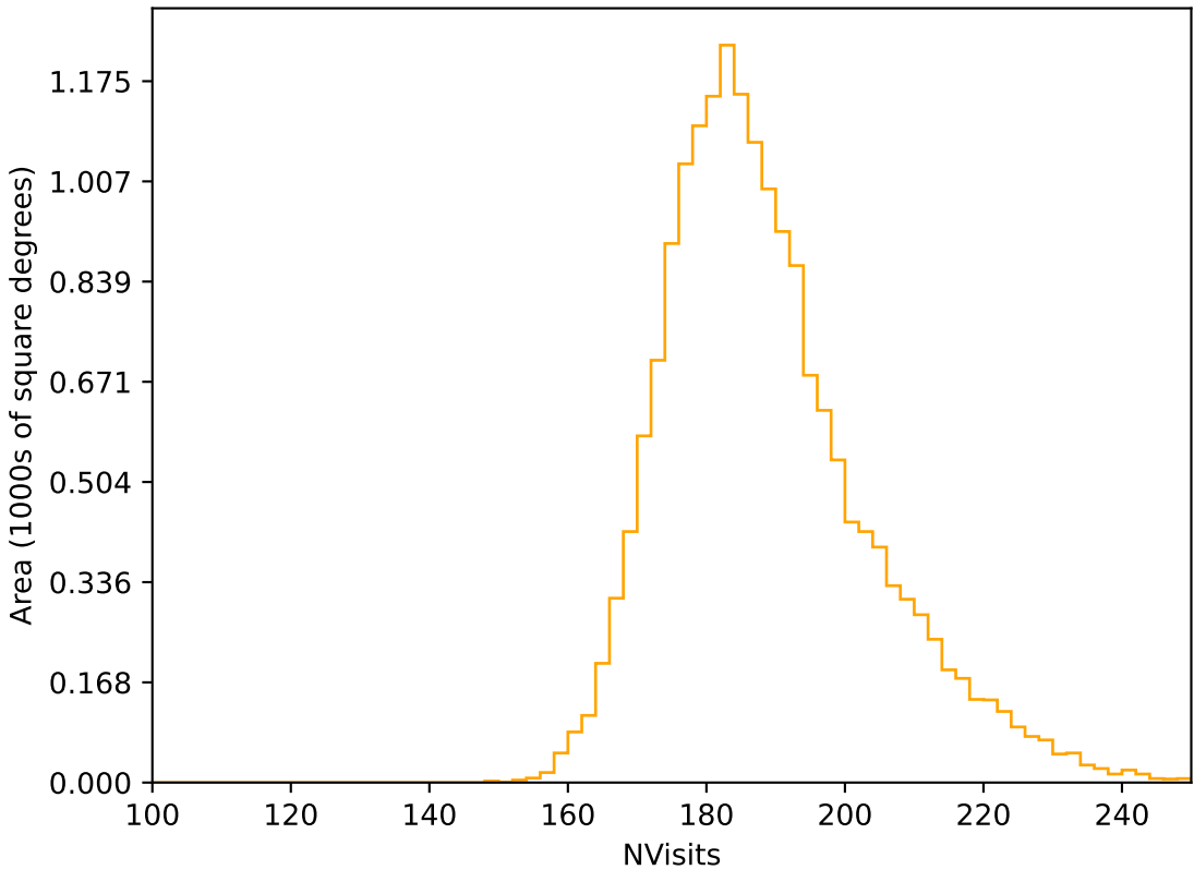
too_elab_heavy_r64_d3_ugrizy_v3.4_10yrs WFD r band: NVisits
