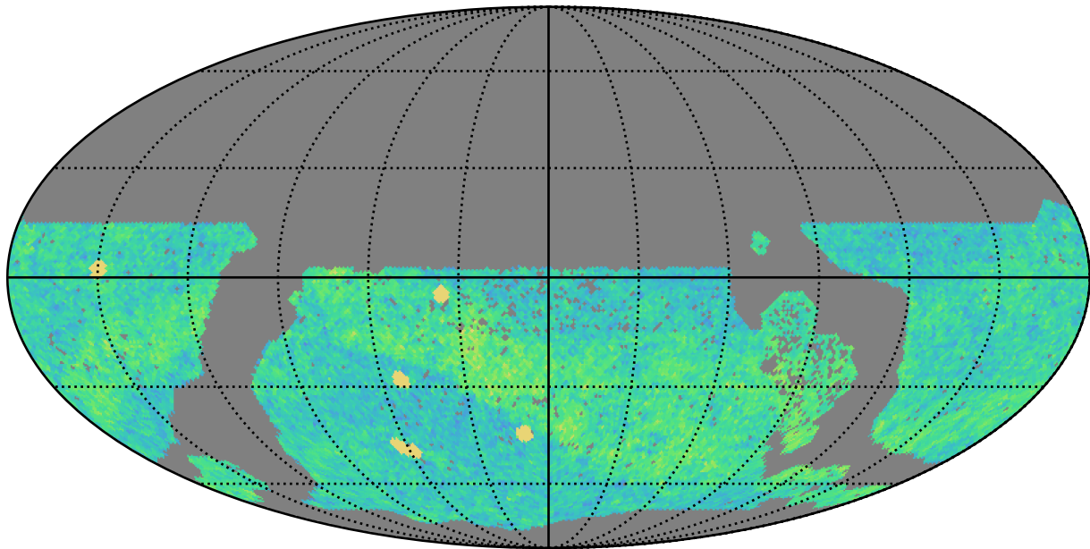
too_elab_heavy_r64_d3_ugrizy_v3.4_10yrs WFD i band: NVisits
