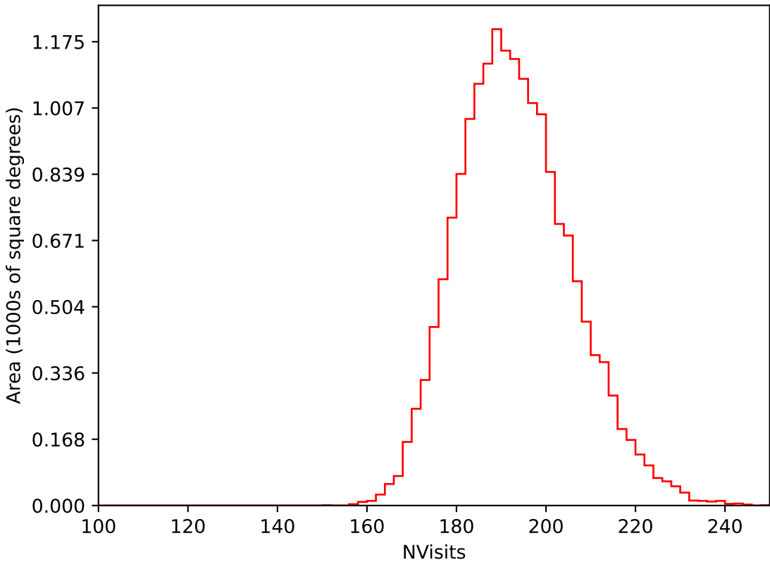
too_elab_heavy_r64_d3_ugrizy_v3.4_10yrs WFD i band: NVisits
