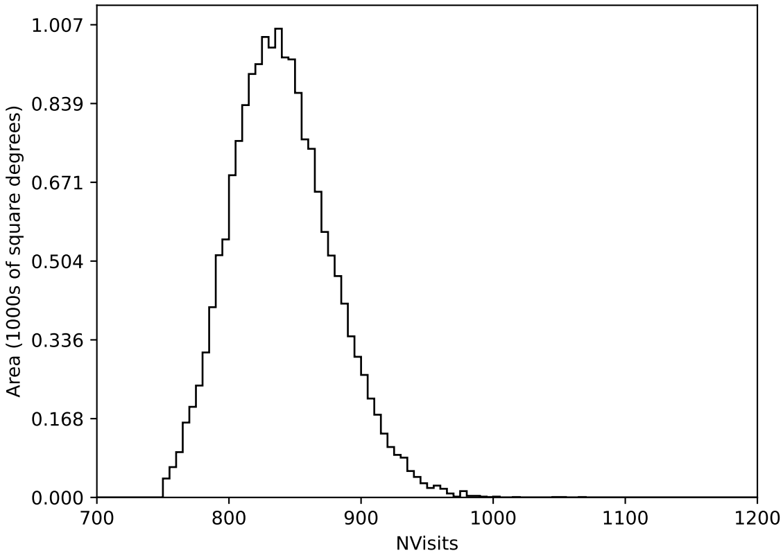
too_elab_heavy_r64_d3_ugrizy_v3.4_10yrs WFD all bands: NVisits
