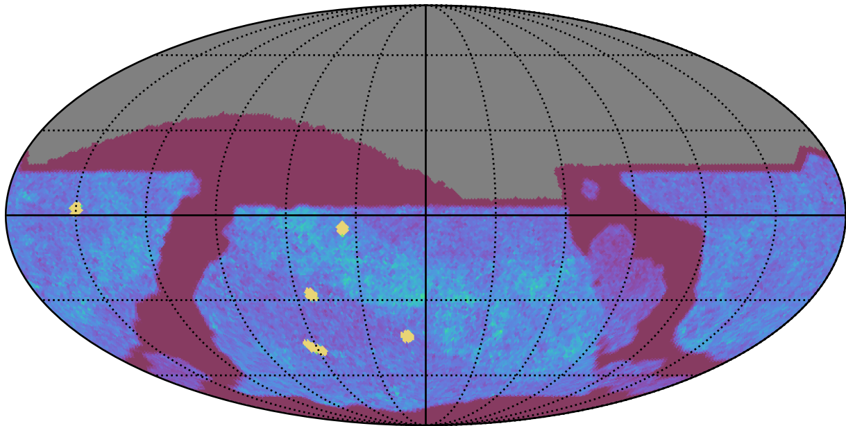
too_elab_heavy_r64_d3_ugrizy_v3.4_10yrs All sky z band: NVisits
