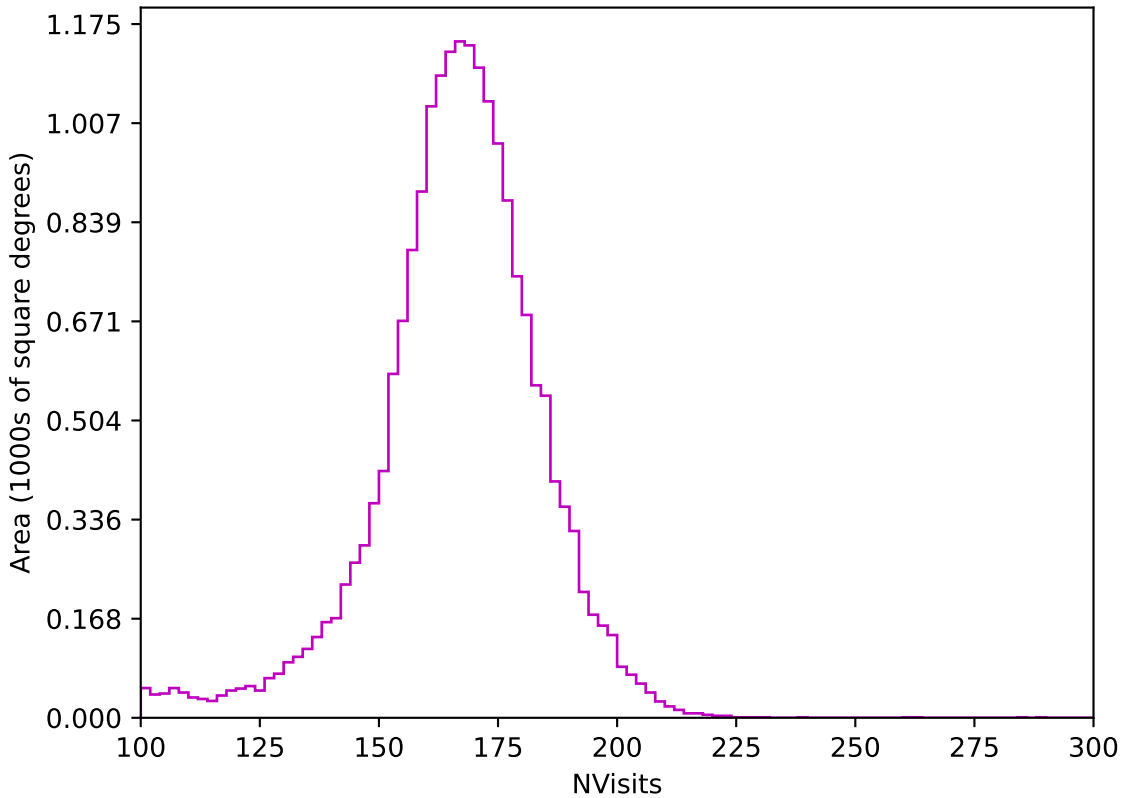
too_elab_heavy_r64_d3_ugrizy_v3.4_10yrs All sky z band: NVisits
