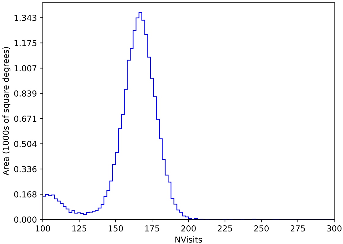
too_elab_heavy_r64_d3_ugrizy_v3.4_10yrs All sky y band: NVisits
