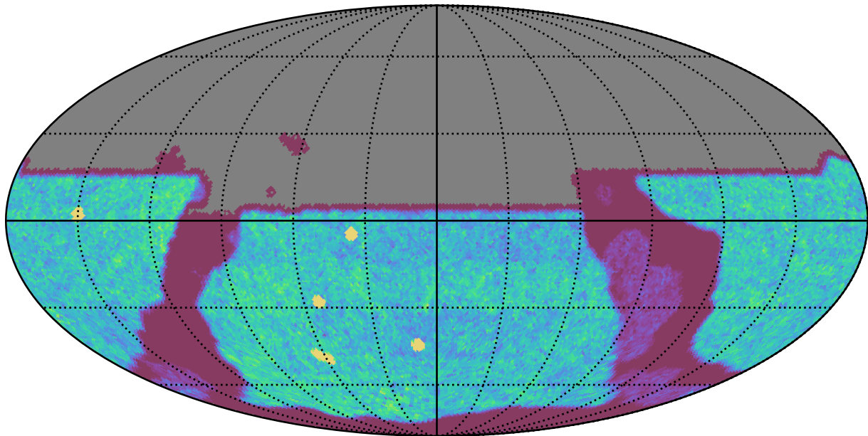
too_elab_heavy_r64_d3_ugrizy_v3.4_10yrs All sky u band: NVisits
