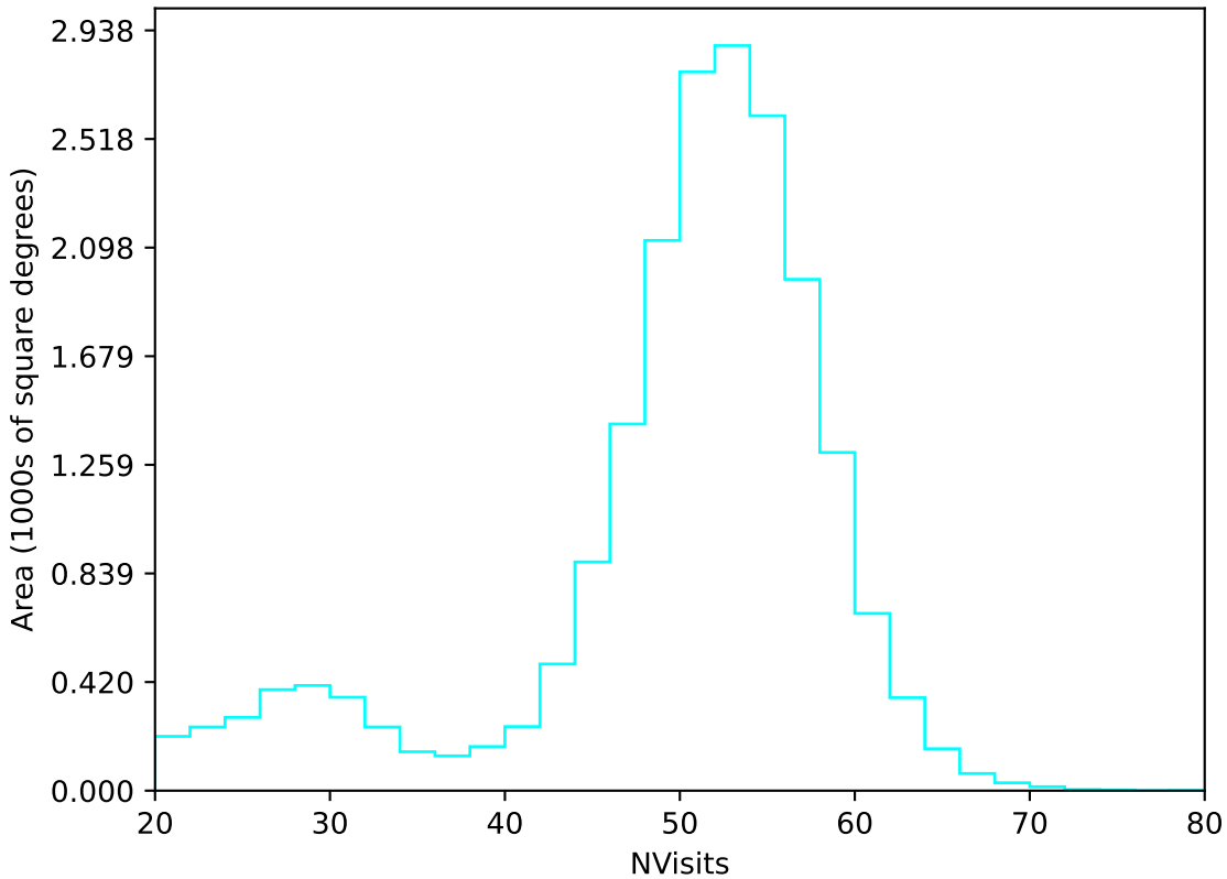
too_elab_heavy_r64_d3_ugrizy_v3.4_10yrs All sky u band: NVisits
