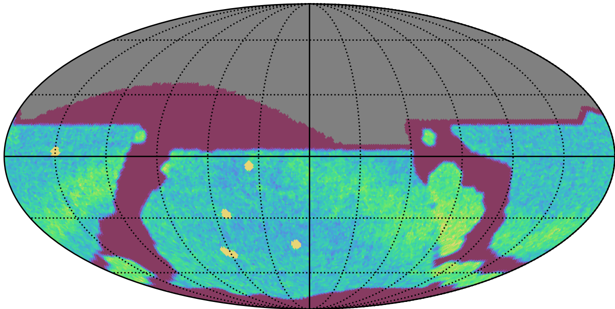
too_elab_heavy_r64_d3_ugrizy_v3.4_10yrs All sky r band: NVisits
