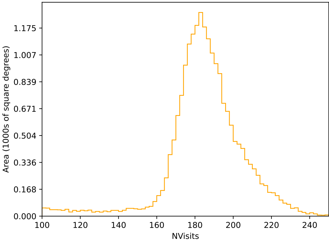
too_elab_heavy_r64_d3_ugrizy_v3.4_10yrs All sky r band: NVisits
