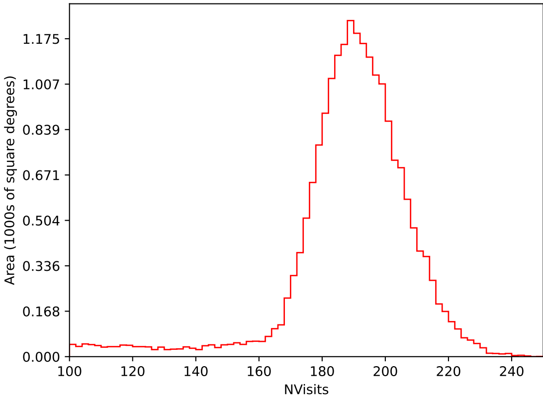
too_elab_heavy_r64_d3_ugrizy_v3.4_10yrs All sky i band: NVisits
