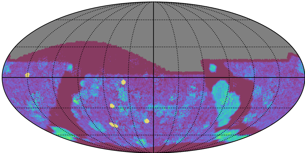
too_elab_heavy_r64_d3_ugrizy_v3.4_10yrs All sky g band: NVisits
