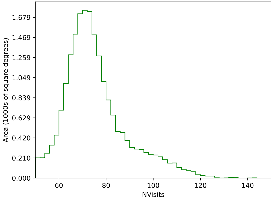
too_elab_heavy_r64_d3_ugrizy_v3.4_10yrs All sky g band: NVisits
