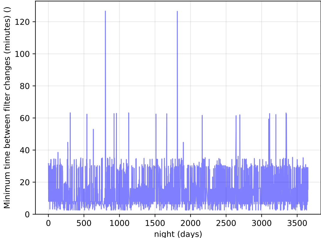
too_elab_heavy_r64_d3_ugrizy_v3.4_10yrs Per Night: Minimum time between filter changes (minutes)
