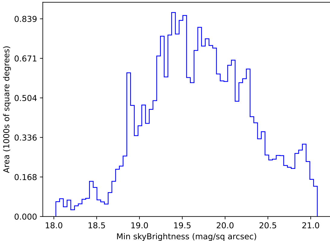
too_elab_heavy_r64_d3_ugrizy_v3.4_10yrs Yr 1 r band: Min skyBrightness
