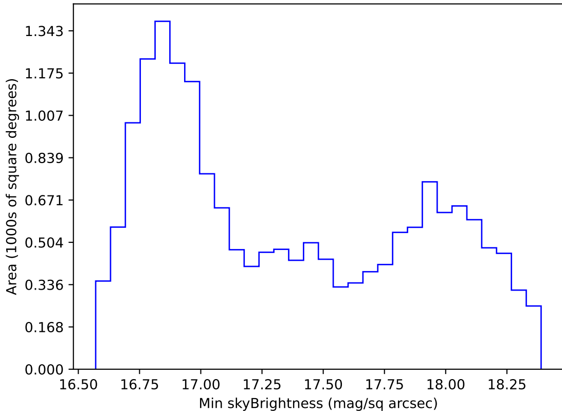
too_elab_heavy_r64_d3_ugrizy_v3.4_10yrs WFD z band: Min skyBrightness
