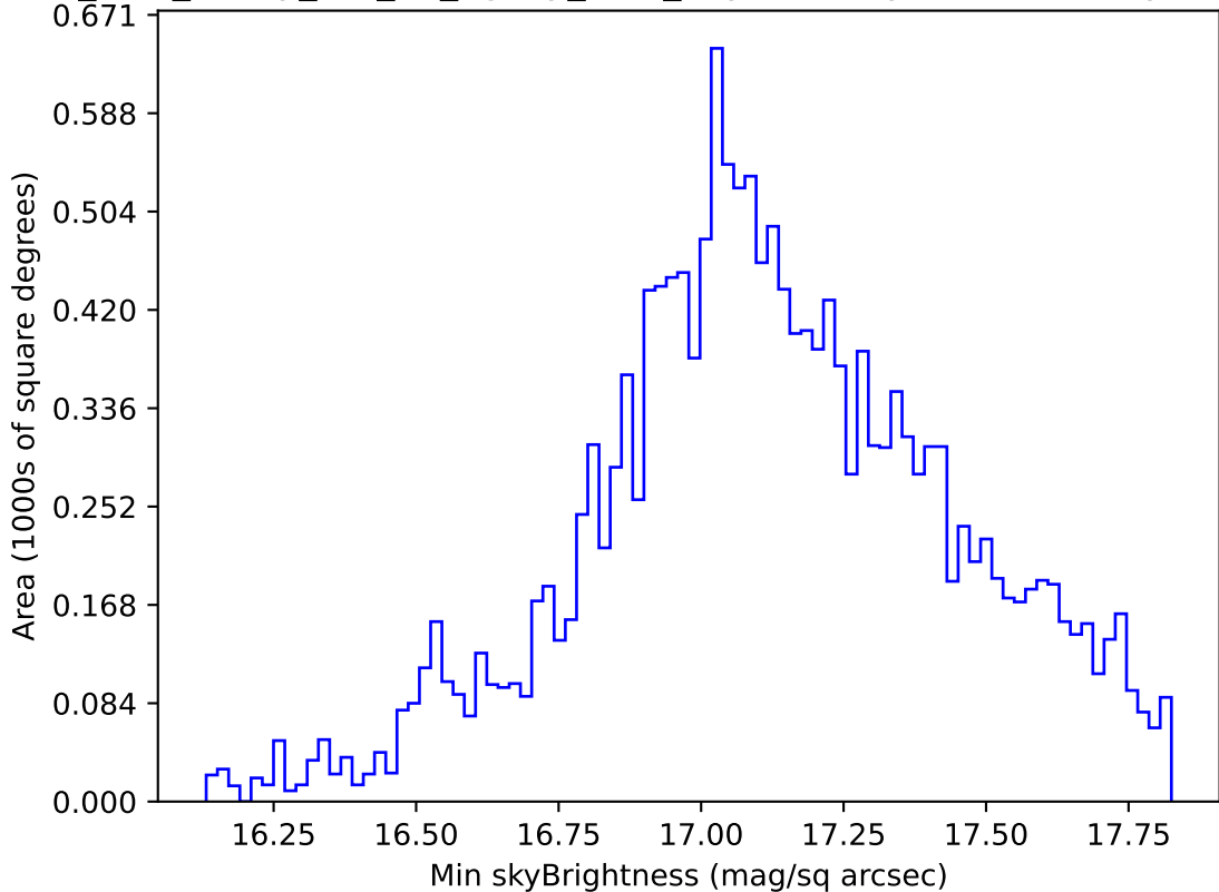
too_elab_heavy_r64_d3_ugrizy_v3.4_10yrs WFD y band: Min skyBrightness
