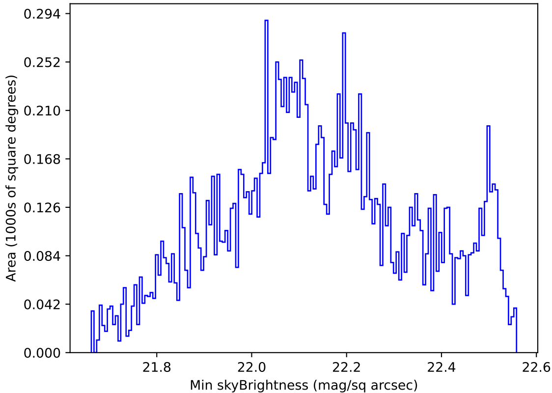
too_elab_heavy_r64_d3_ugrizy_v3.4_10yrs WFD u band: Min skyBrightness
