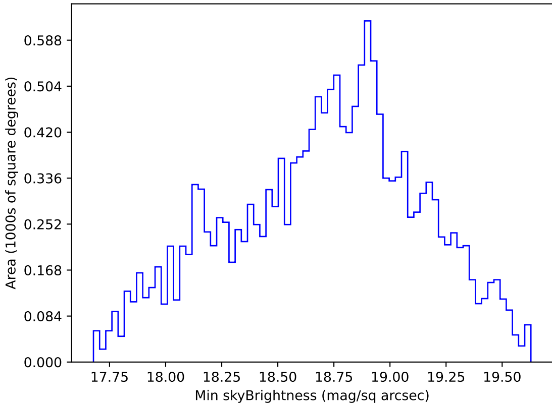
too_elab_heavy_r64_d3_ugrizy_v3.4_10yrs WFD r band: Min skyBrightness
