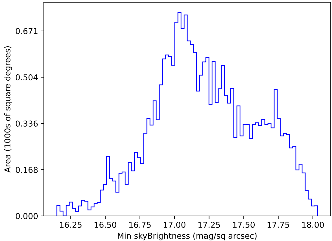
too_elab_heavy_r64_d3_ugrizy_v3.4_10yrs All sky y band: Min skyBrightness
