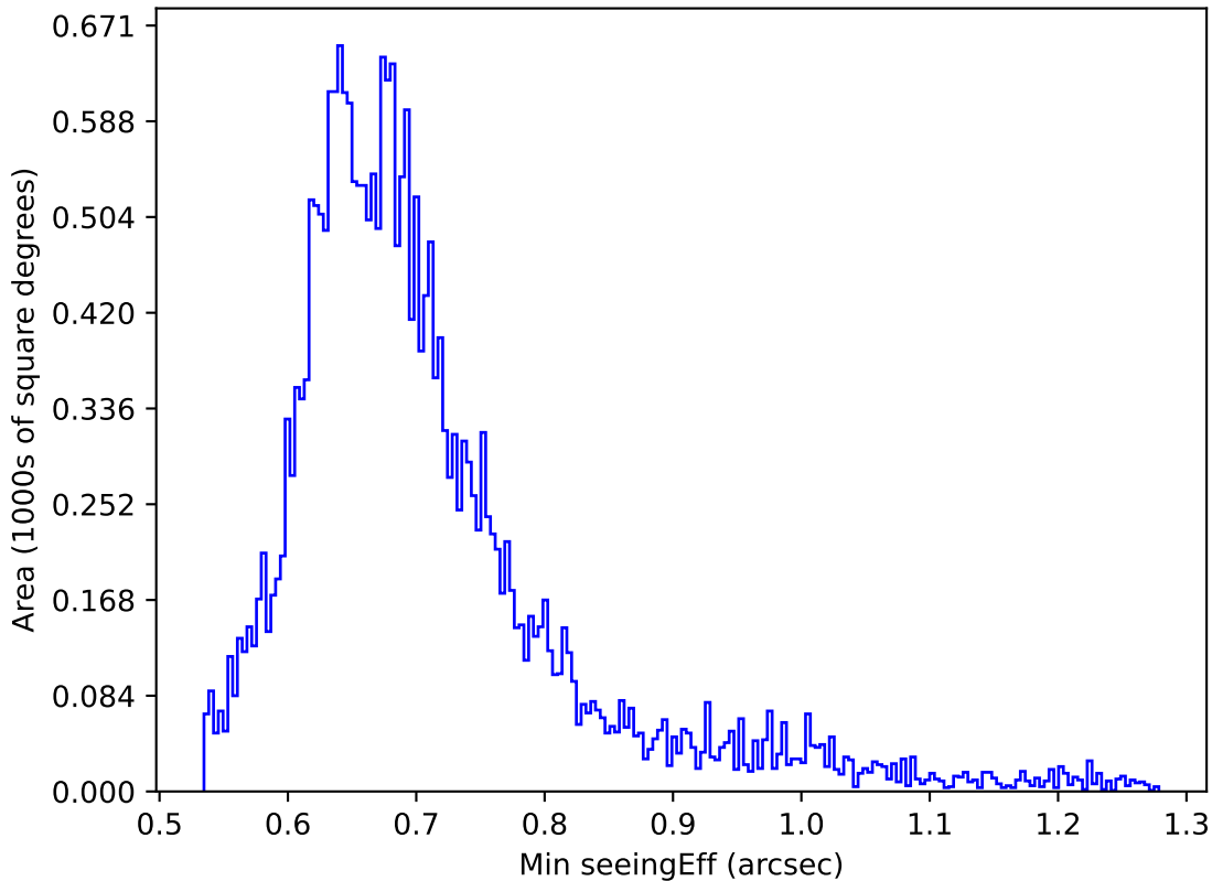
too_elab_heavy_r64_d3_ugrizy_v3.4_10yrs Yr 1 i band: Min seeingEff
