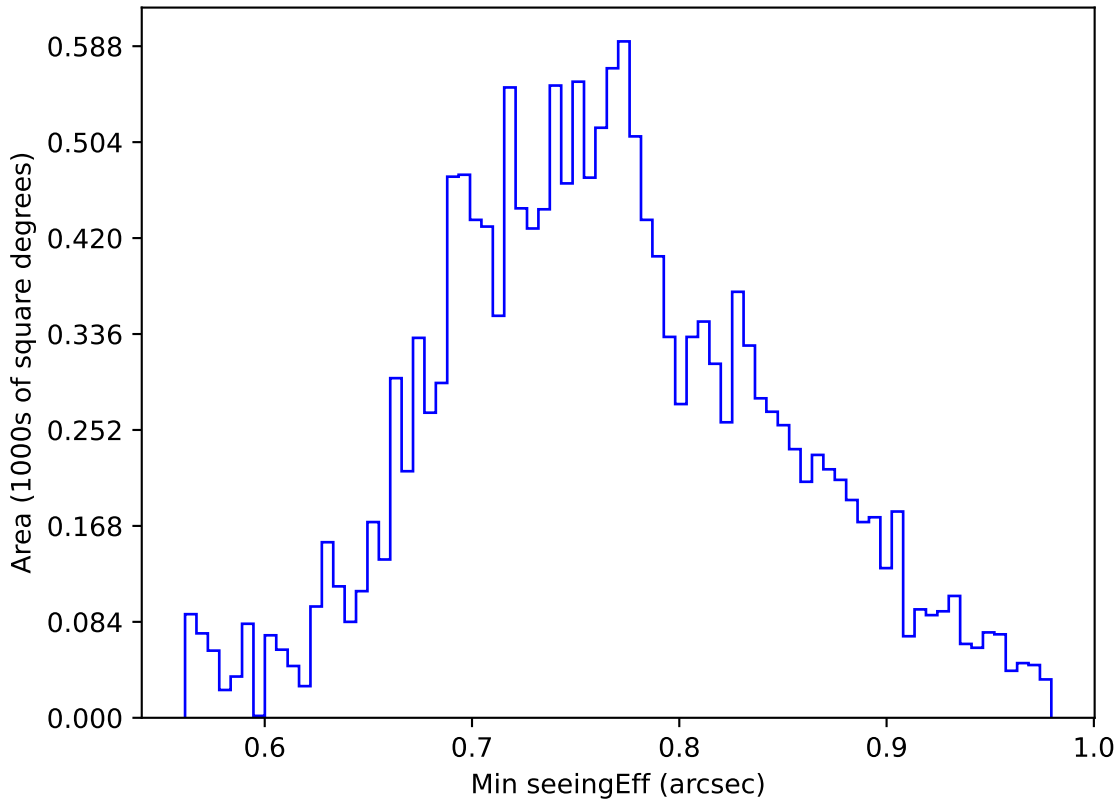
too_elab_heavy_r64_d3_ugrizy_v3.4_10yrs WFD u band: Min seeingEff
