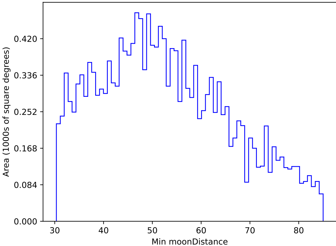
too_elab_heavy_r64_d3_ugrizy_v3.4_10yrs WFD u band: Min moonDistance
