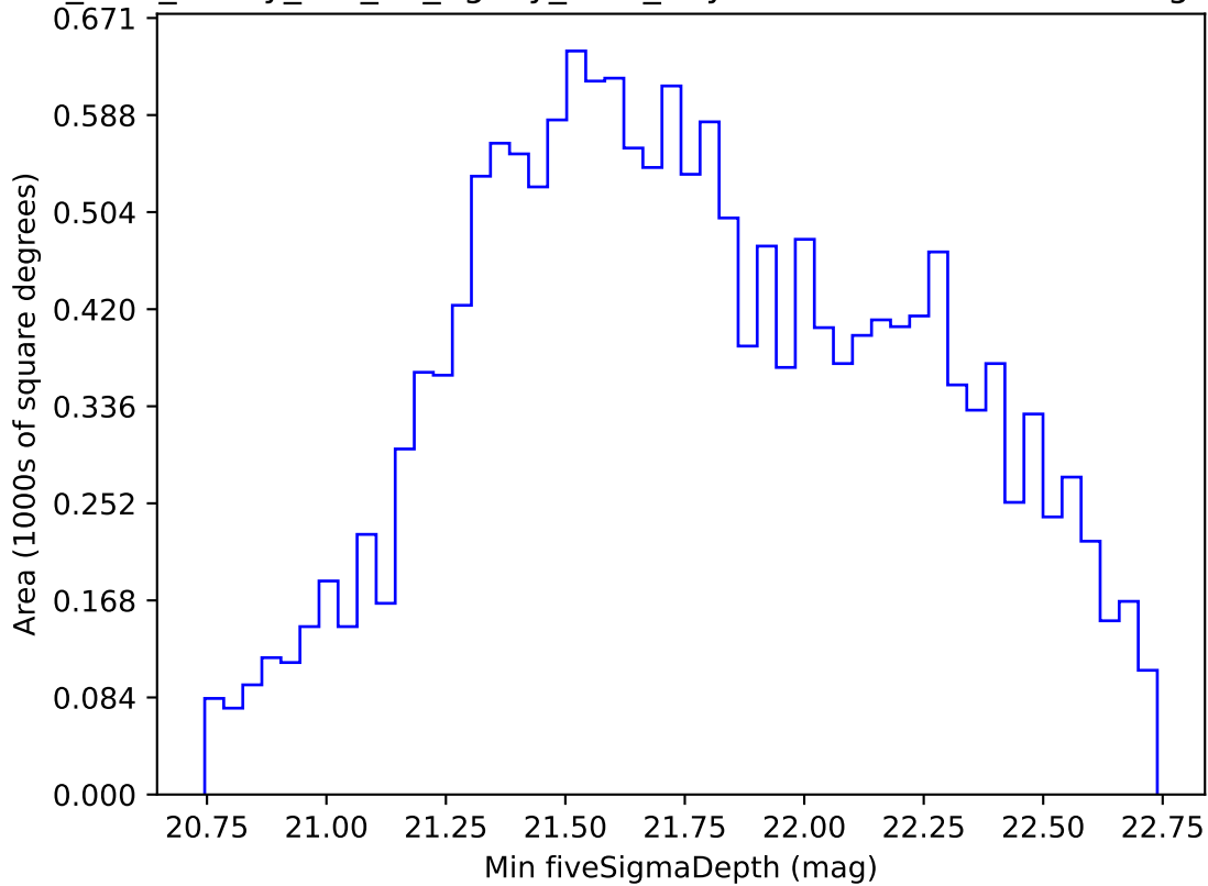
too_elab_heavy_r64_d3_ugrizy_v3.4_10yrs WFD i band: Min fiveSigmaDepth
