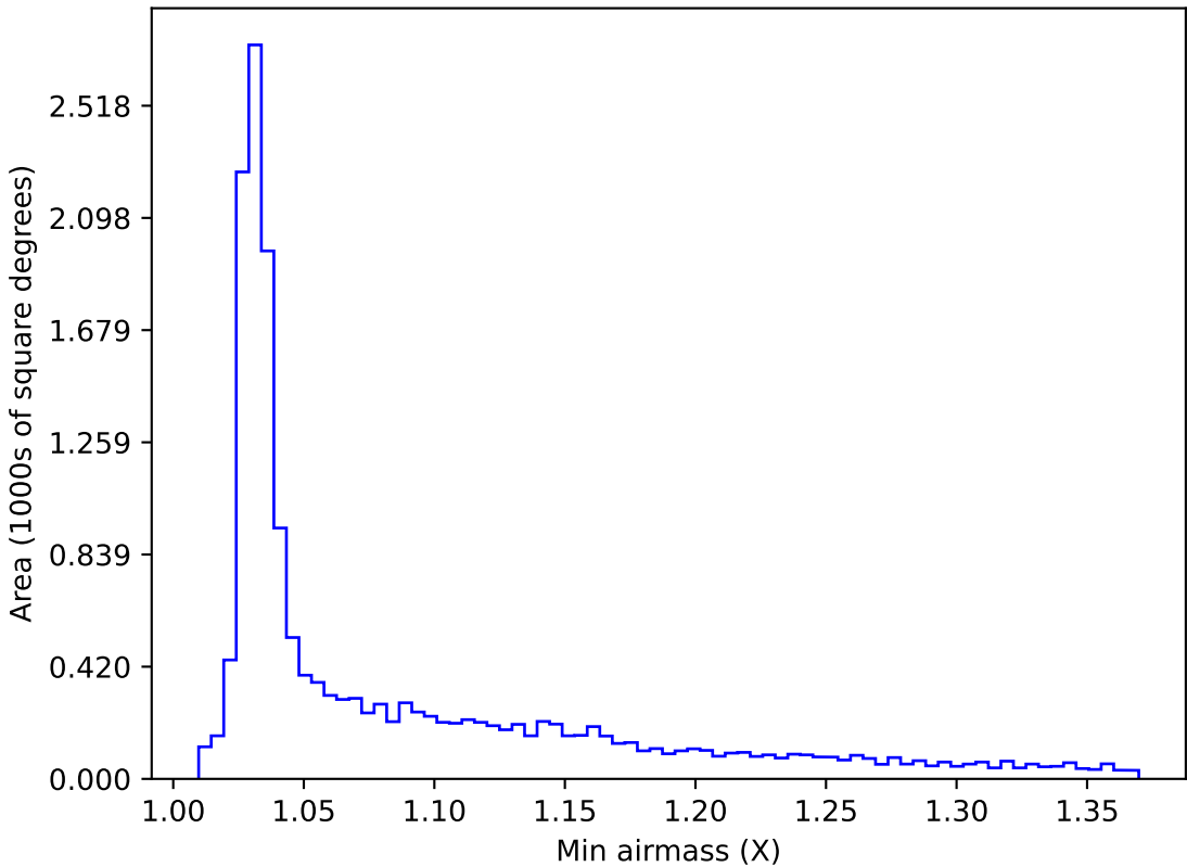
too_elab_heavy_r64_d3_ugrizy_v3.4_10yrs WFD y band: Min airmass
