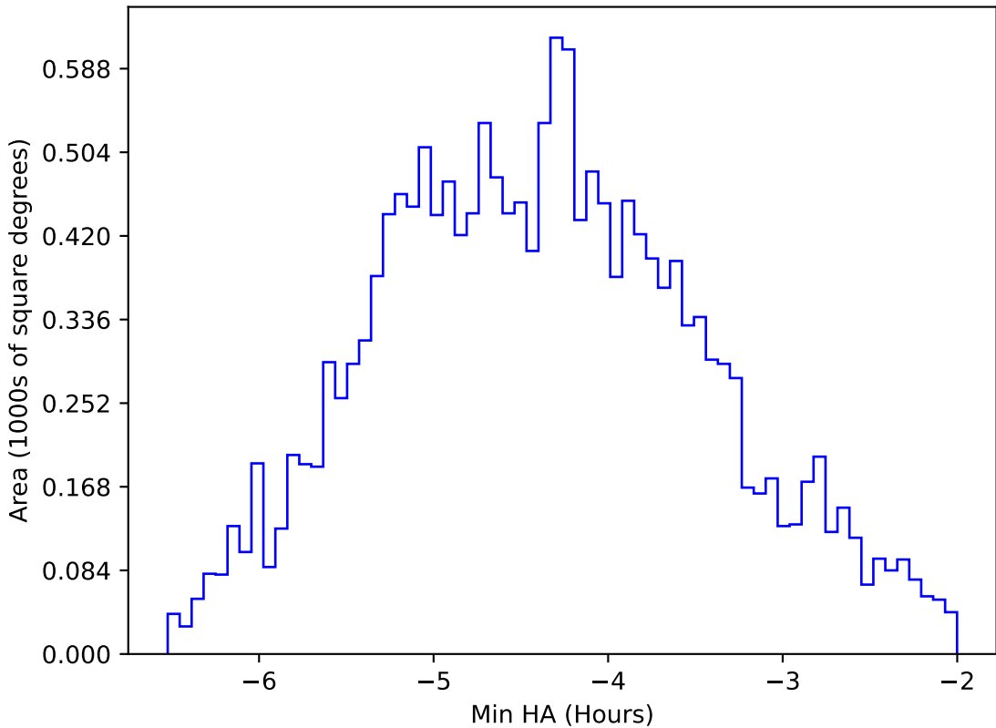
too_elab_heavy_r64_d3_ugrizy_v3.4_10yrs WFD z band: Min HA
