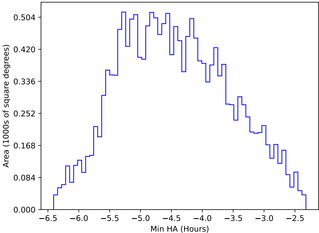
too_elab_heavy_r64_d3_ugrizy_v3.4_10yrs WFD r band: Min HA
