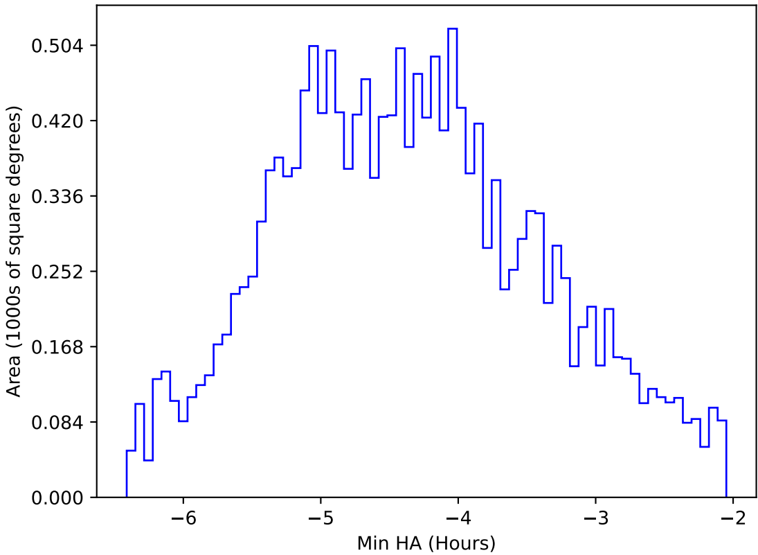
too_elab_heavy_r64_d3_ugrizy_v3.4_10yrs WFD i band: Min HA
