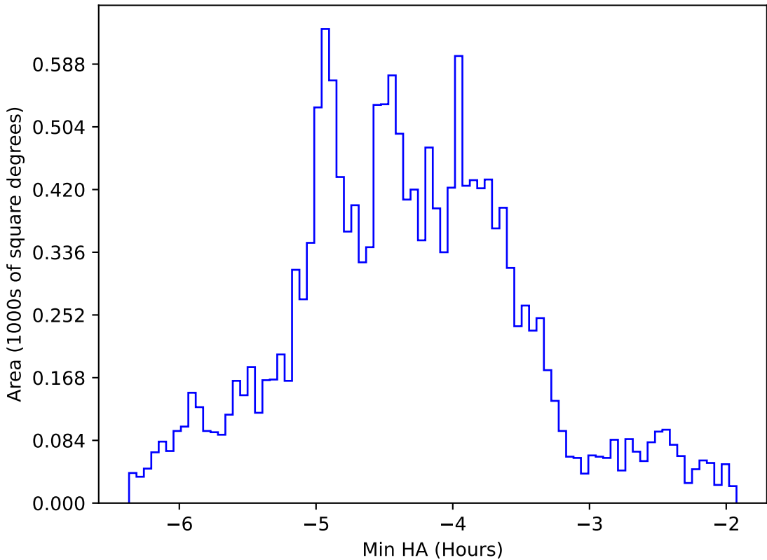
too_elab_heavy_r64_d3_ugrizy_v3.4_10yrs WFD g band: Min HA
