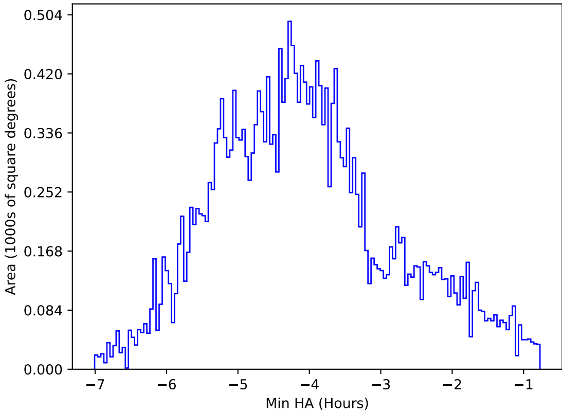
too_elab_heavy_r64_d3_ugrizy_v3.4_10yrs All sky z band: Min HA
