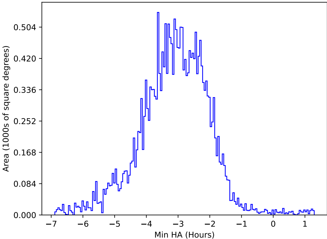
too_elab_heavy_r64_d3_ugrizy_v3.4_10yrs All sky u band: Min HA
