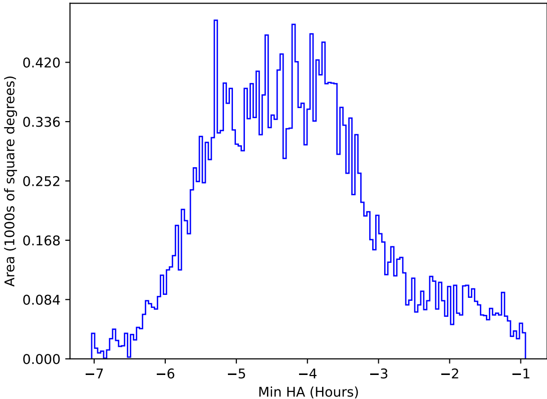
too_elab_heavy_r64_d3_ugrizy_v3.4_10yrs All sky r band: Min HA
