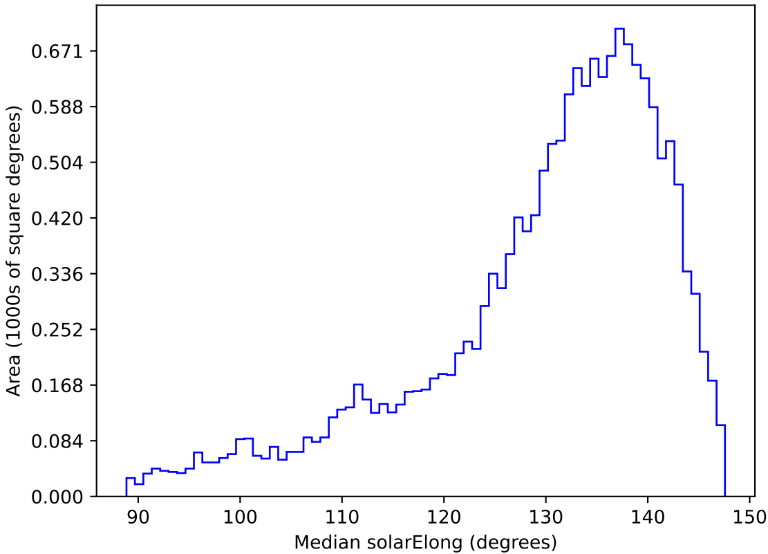
too_elab_heavy_r64_d3_ugrizy_v3.4_10yrs WFD y band: Median solarElong
