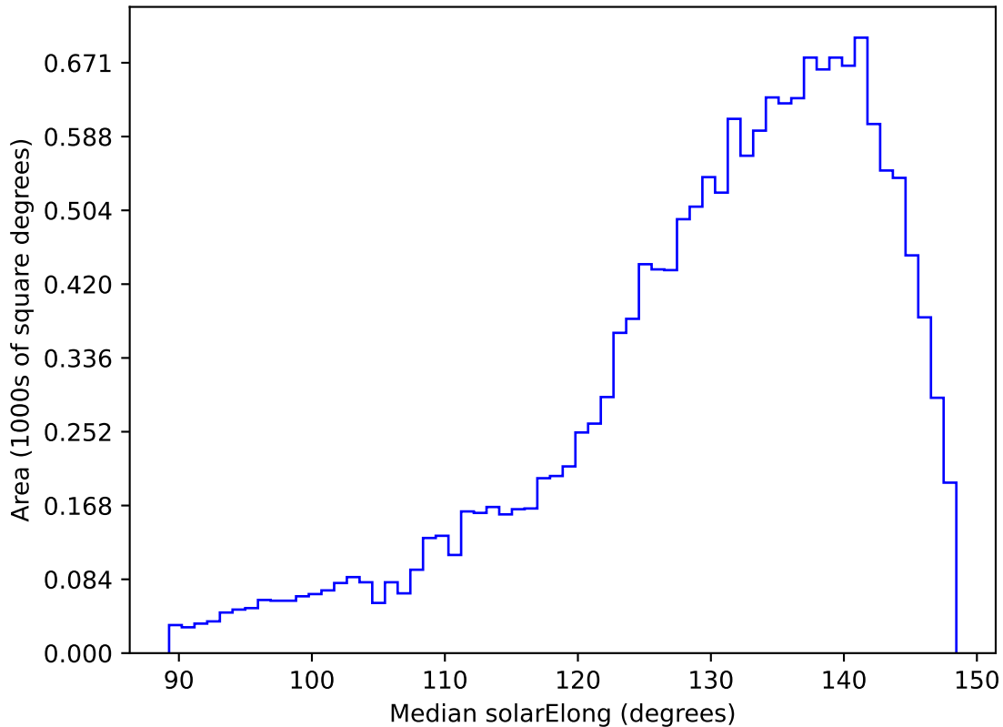
too_elab_heavy_r64_d3_ugrizy_v3.4_10yrs WFD r band: Median solarElong
