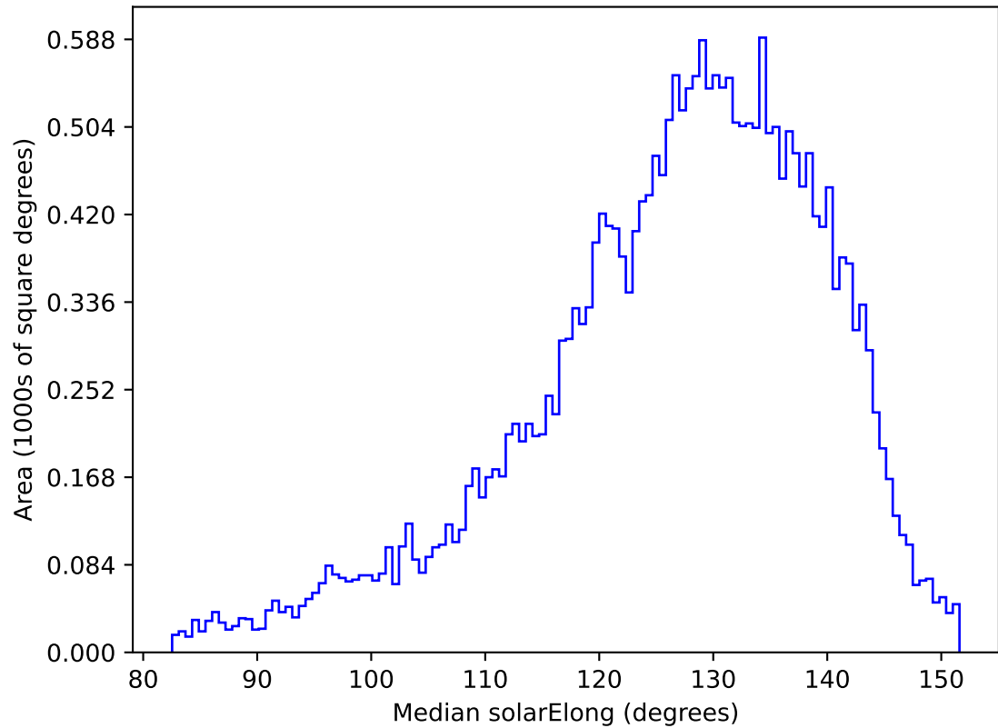
too_elab_heavy_r64_d3_ugrizy_v3.4_10yrs All sky z band: Median solarElong
