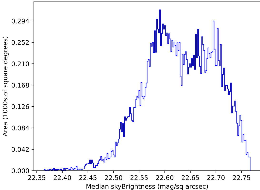
too_elab_heavy_r64_d3_ugrizy_v3.4_10yrs Yr 1 u band: Median skyBrightness
