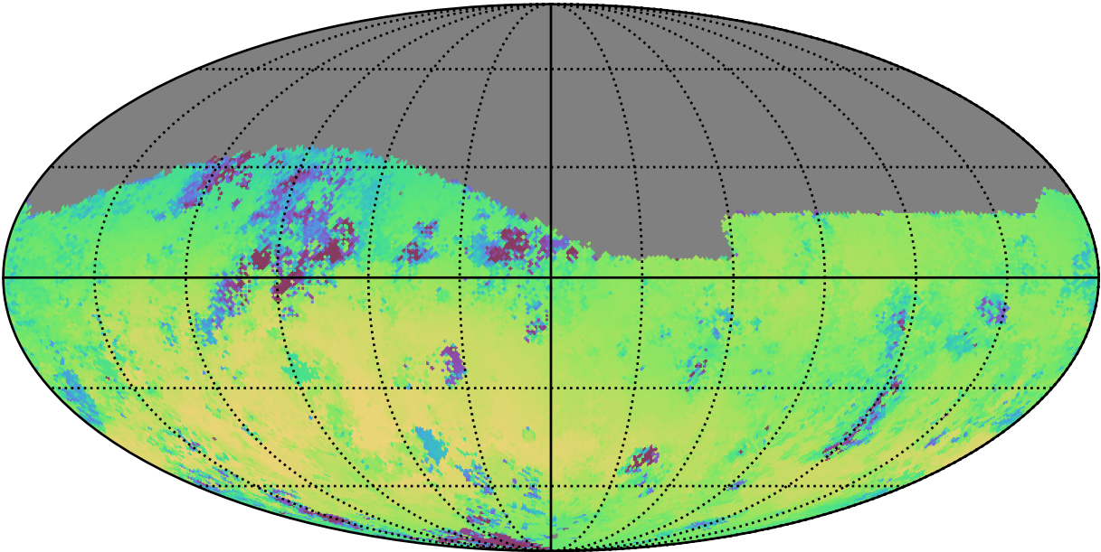
too_elab_heavy_r64_d3_ugrizy_v3.4_10yrs Yr 1 r band: Median skyBrightness
