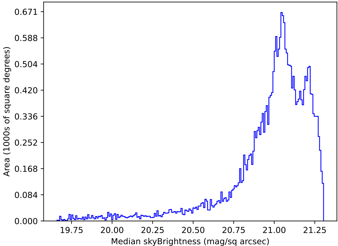
too_elab_heavy_r64_d3_ugrizy_v3.4_10yrs Yr 1 r band: Median skyBrightness
