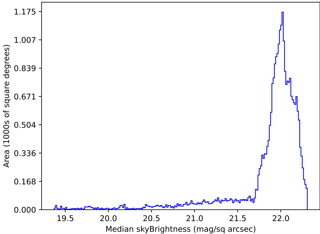
too_elab_heavy_r64_d3_ugrizy_v3.4_10yrs Yr 1 g band: Median skyBrightness
