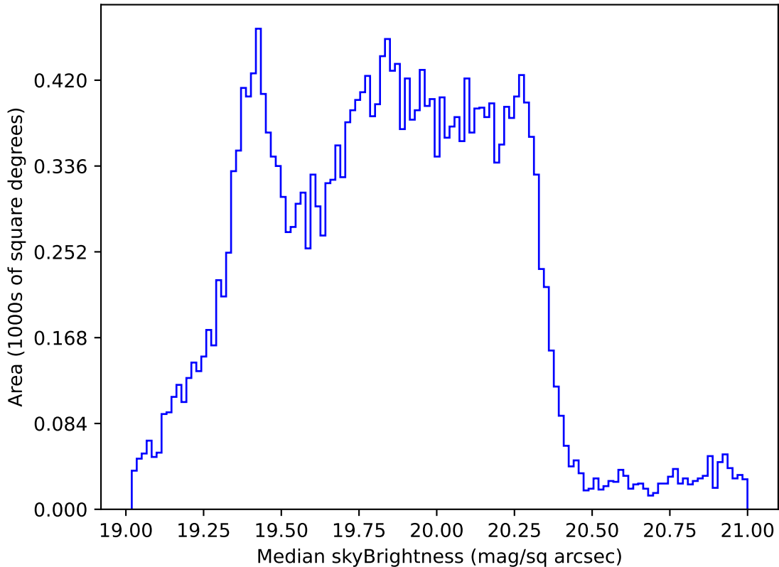
too_elab_heavy_r64_d3_ugrizy_v3.4_10yrs Yr 1 all bands: Median skyBrightness
