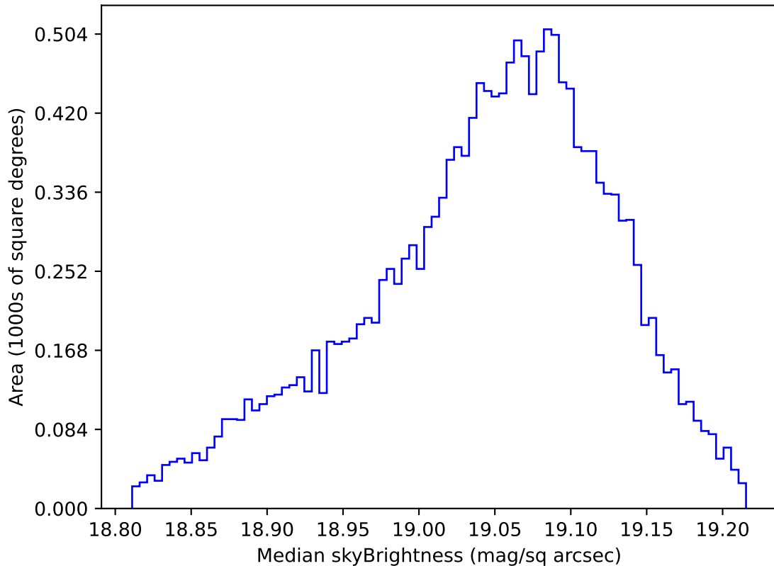
too_elab_heavy_r64_d3_ugrizy_v3.4_10yrs WFD z band: Median skyBrightness
